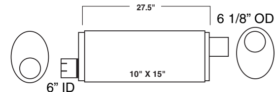
MODEL: CAT 988, 824B, 826B 8S6443
