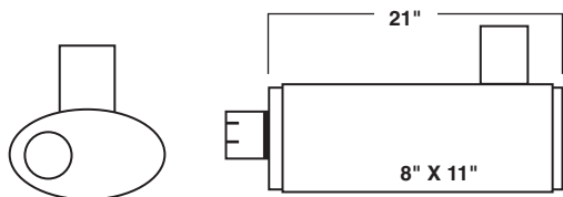
(ALSO ON PAGE OR10) MODEL: CAT 215 EXCAVATOR 6C0482
